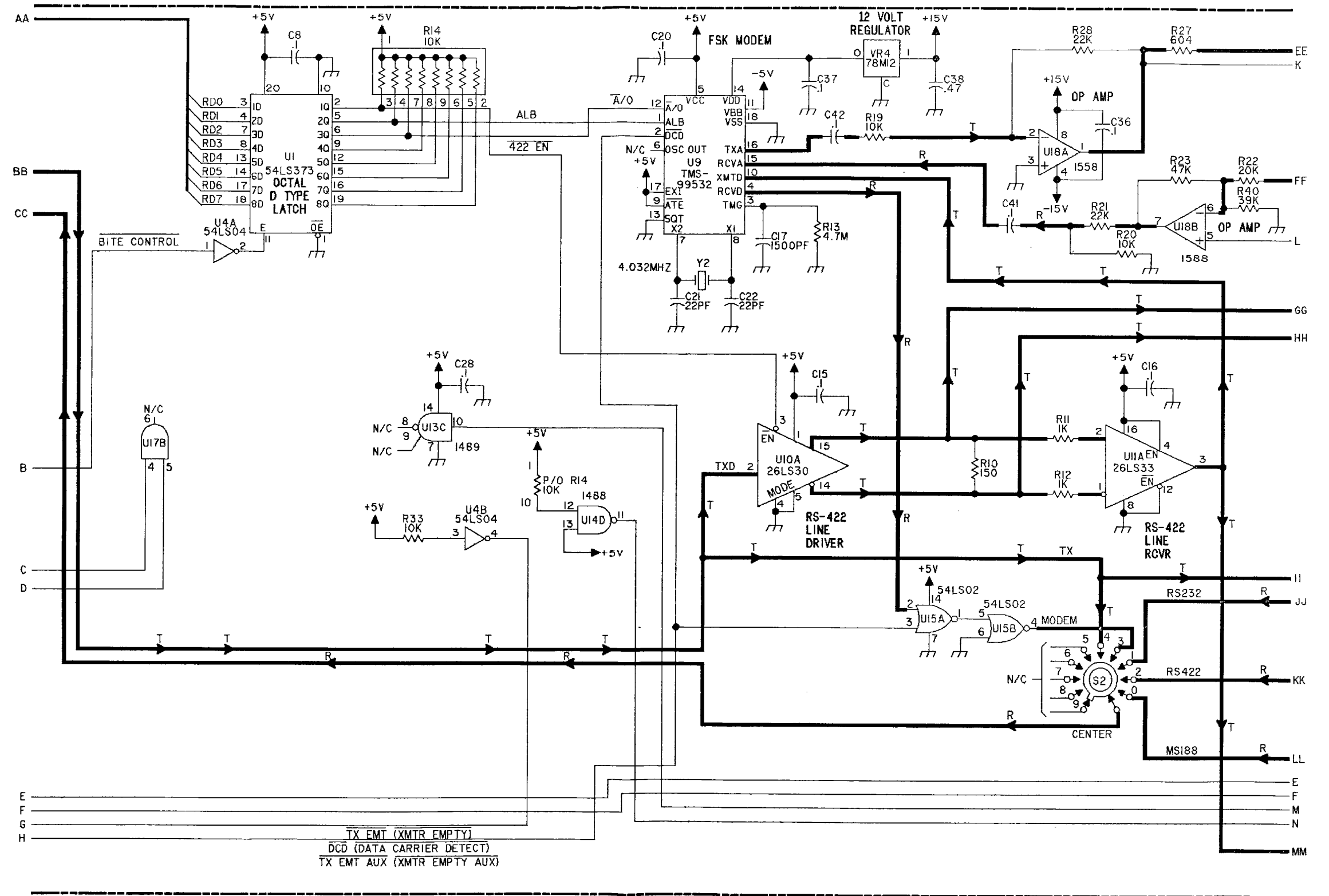
FO-9. Remote Control Interface PWB Assy, A1A19 (in Transceiver) (Sheet 2 of 3)
