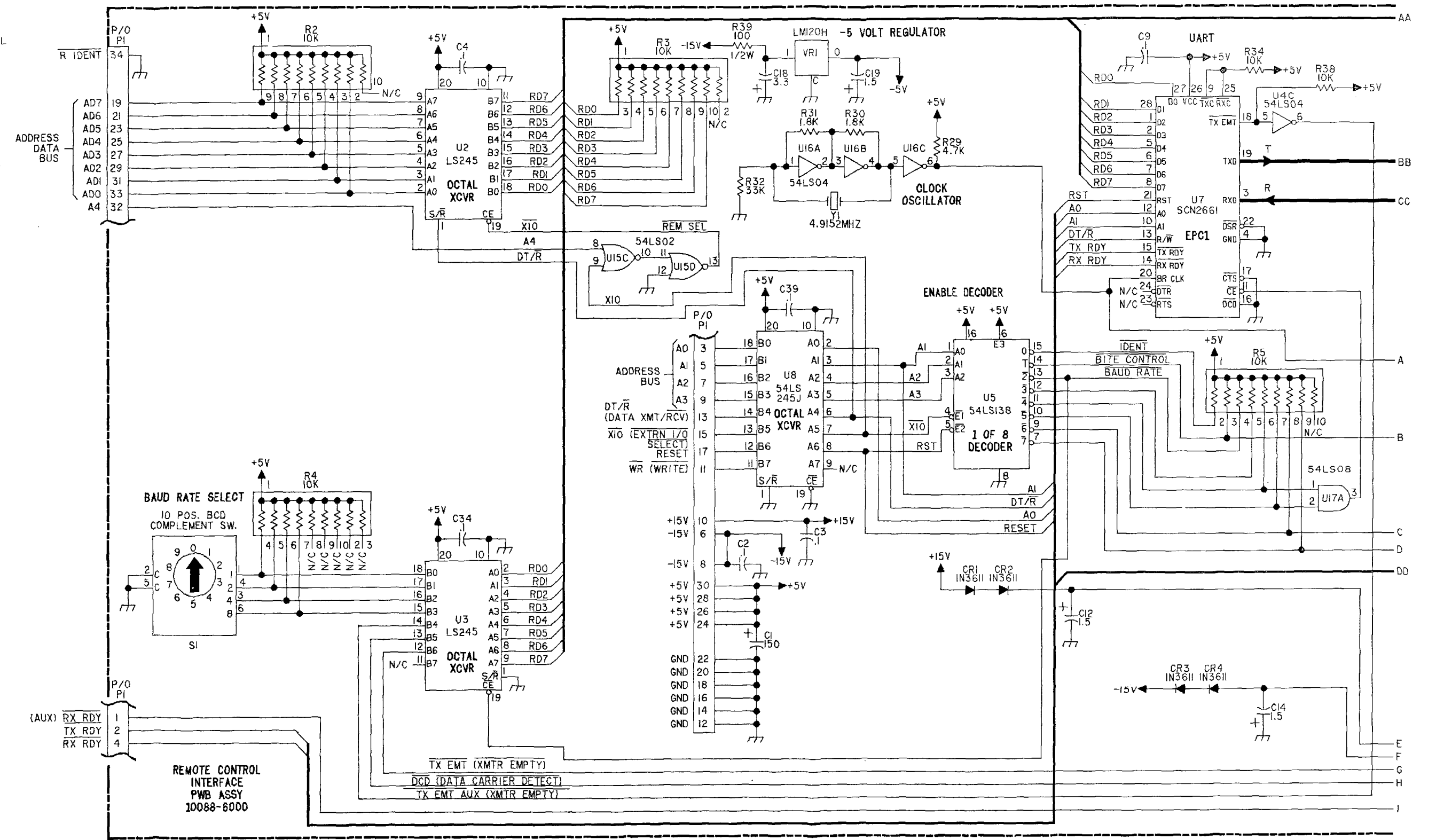
FO-9. Remote Control Interface PWB Assy, A1A19 (in Transceiver) (Sheet 1 of 3)
